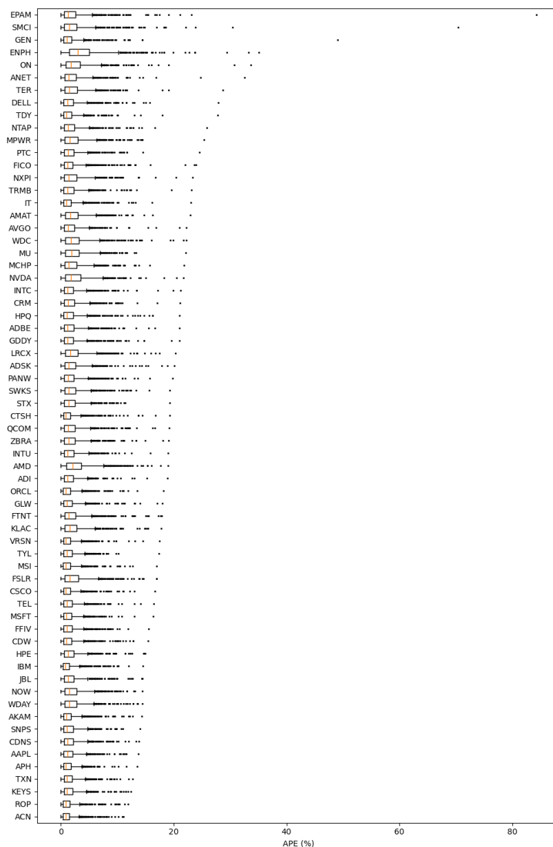
Figure 3.9: Distribution of APE for single stocks on training-validation interval (General model Ridge).
