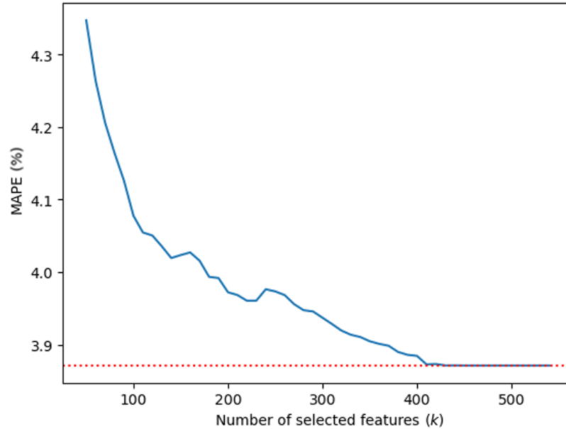
Figure 3.1: MAPE dependence on number of features selected (Linear regression, stock ENPH).
